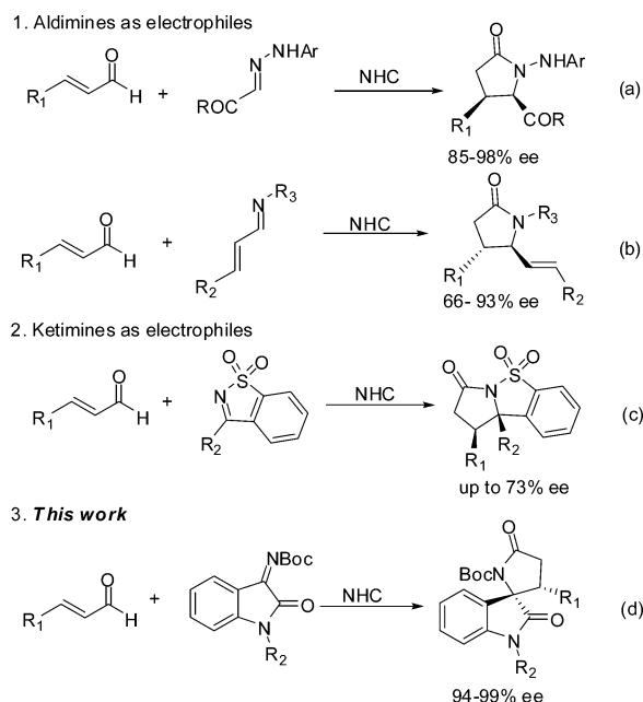
Scheme 1. Asymmetric Synthesis of \gamma -Lactams via NHC Catalysis
