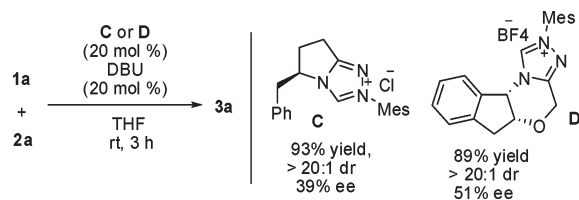
Scheme 1. Enantioselective Synthesis of 3a
