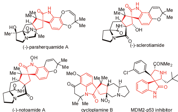
Figure 1. Examples of natural products and synthetic inhibitors containing spiro oxindole scaffolds.
