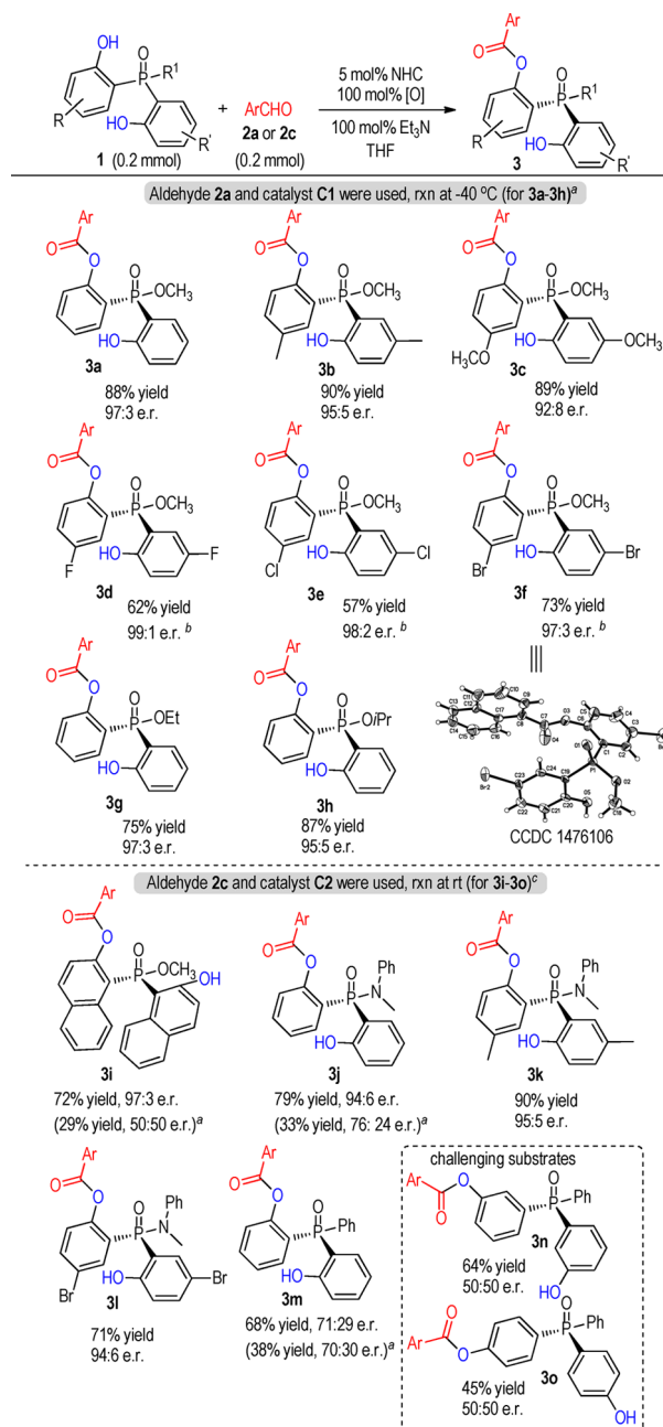
Chart 1. Substrate Scope
