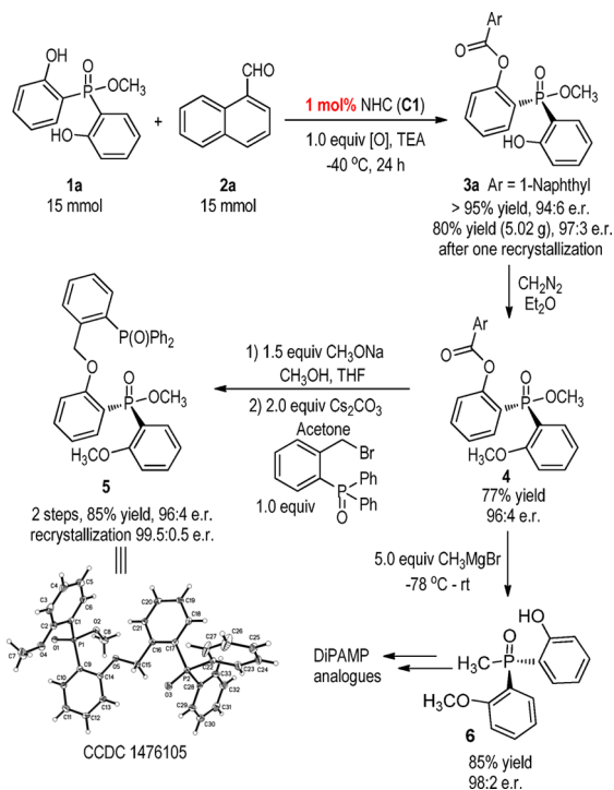
Scheme 2. Synthetic Transformations
