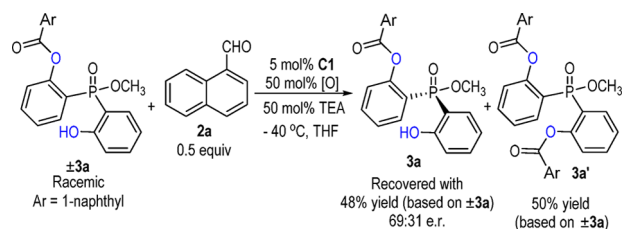
Scheme 3. Kinetic Resolution Is Not a Main Contributor to the Observed Enantioselectivity
