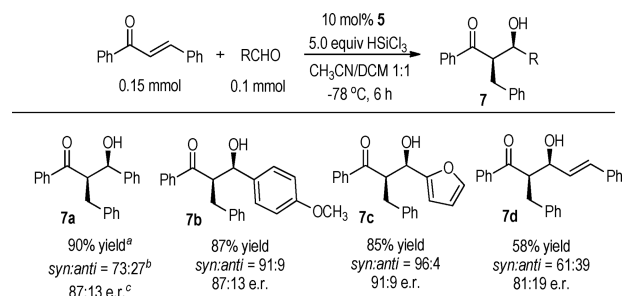
Chart 2. Application of P-Stereogenic Phosphinate 5 as a Catalyst
