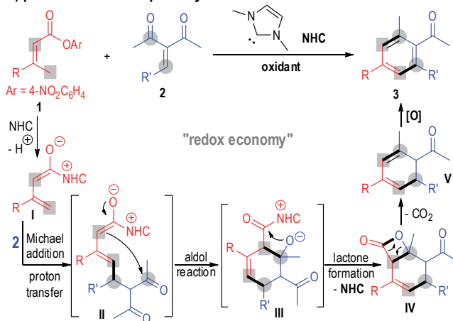
Figure 1 NHC-catalyzed ester activation for benzene synthesis.
