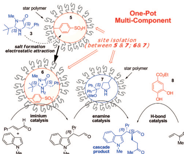
Figure 1. Illustration of our design: non-interpenetrating star polymers for one-pot cascade catalysis.
