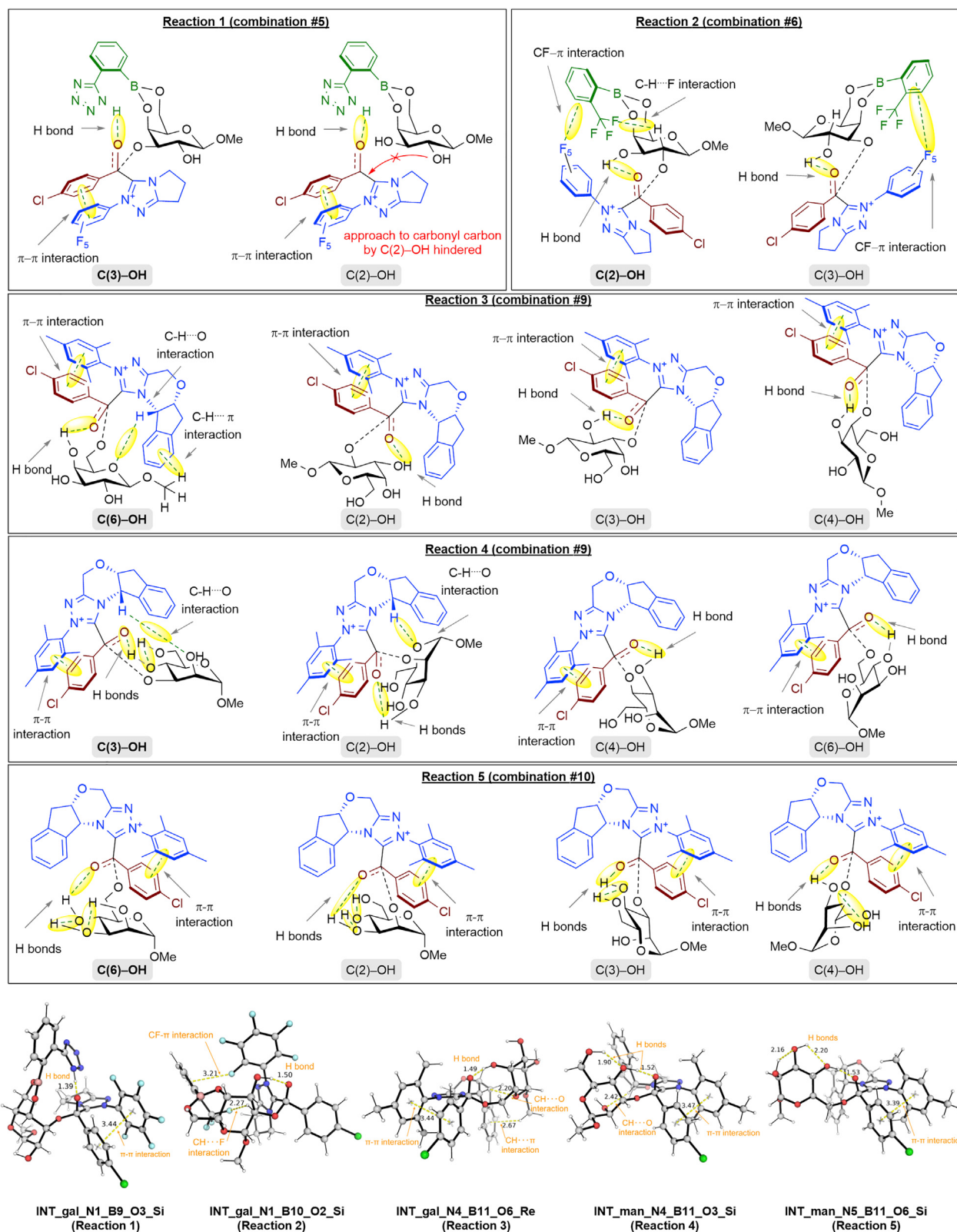
Figure 6. Schematic representation of the NCIs involved in the key regioselective step for model reactions considered by DFT calculations
