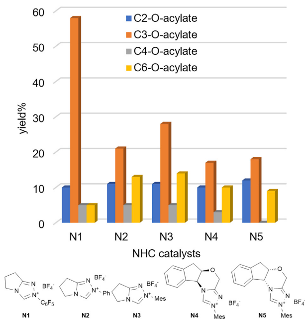
Figure 3. Conditions for site-selective acylation of a model saccharide as mediated by NHC catalysts and boronic acids
