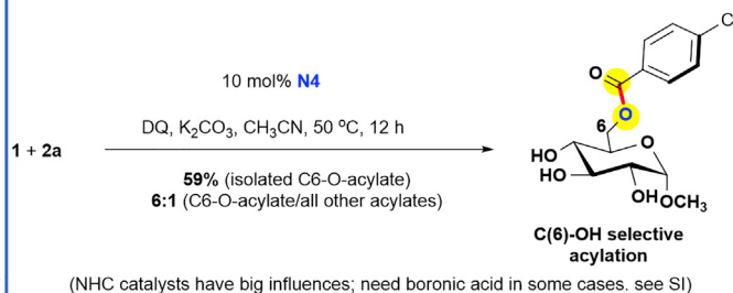
Figure 3. Conditions for site-selective acylation of a model saccharide as mediated by NHC catalysts and boronic acids
