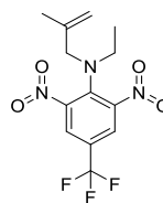
Ethalfuralin
