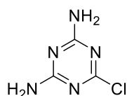
1,3,5-Triazine-2,4-diamine, 6-chloro-
