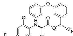
Tau-fluvalinate
