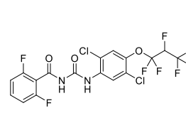
Lufenuron
