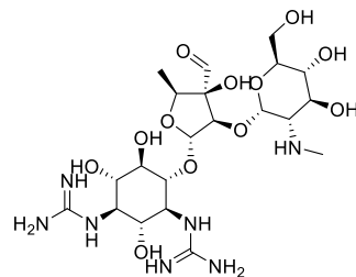
streptomycin
