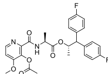
Florypicoxamid
