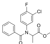
Flamprop-methyl
