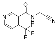
Flonicamid
