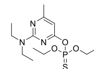
Pirimiphos ethyl
