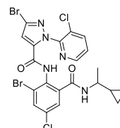
Cyclaniliprole
