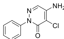
Chlordinon
