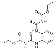
thiophanate
