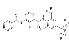
Broflanilide
