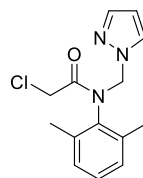
Metazachlor
