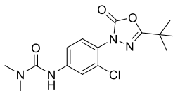
Dimefuron
