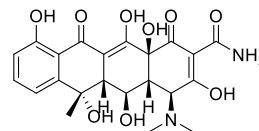
oxytetracycline
