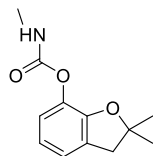
Carbofuran
