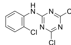
anilazine
