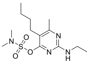
bupirimate
