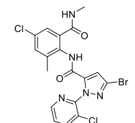
Chlorantraniliprole
