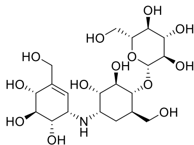
validamycin
