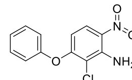
Aclonifen
