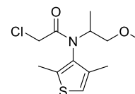
Dimethenamid
