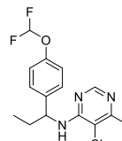
diflumetorim
