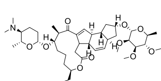
Spinosad
