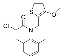
Thenylchlor
