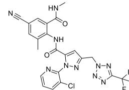
Tetraniliprole
