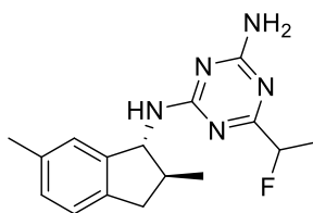
Indaziflam
