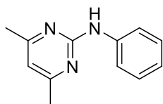
pyrimethanil
