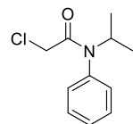
Propachlor
