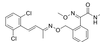
fenaminstrobin
