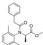
benalaxyl-M
