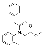
benalaxyl
