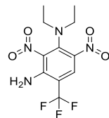
Dinitramine
