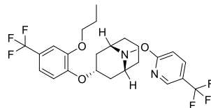
1332838-17-1 氟螞啉 (acynonapyr)
